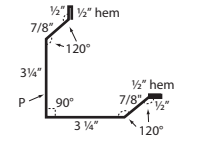
10 Inside Corner Trim PF06
