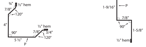
8 4 1/2" Drip Cap PF15
