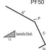
20b Notched Gambrel Flashing (41") PF50
