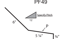
19b Notched Transition Flashing (41") PF49
