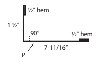
16a End Wall PF08
