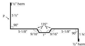
20a Gambrel Flashing PF11
