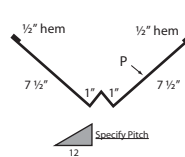
21 Preformed Valley PF12
