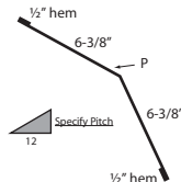
20a Gambrel Flashing PF11
